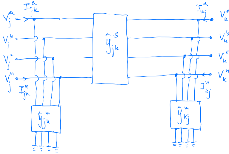
Figure 8.1: A four-wire line characterized by 4 \times 4 series and shunt admittance matrices (\hat{y}_{jk}^S, \hat{y}_{jk}^m, \hat{y}_{kj}^m) .
