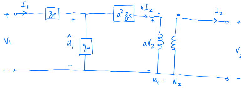
Figure 3.34: Example 3.1: T equivalent circuit of transformer with n := N_2/N_1 and a := N_1/N_2 .
