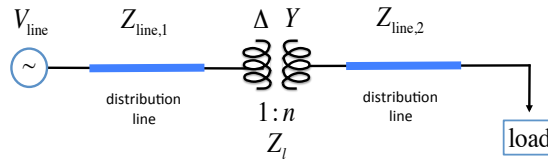
Figure 3.41: The three-phase transformer is connected to a three-phase voltage source and a three-phase load through two three-phase lines.
