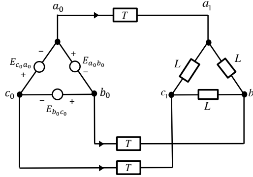
Figure 1.17: Example 1.5. (Fig change: T \rightarrow t , L \rightarrow l .)
