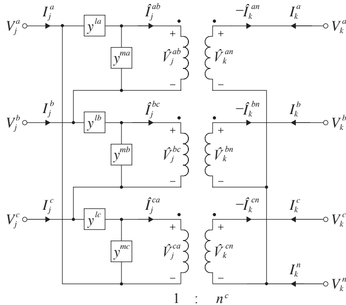
Figure 8.14: \Delta Y -configured transformer.
