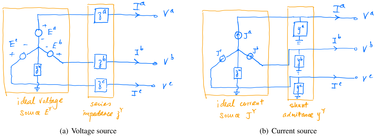
Figure 8.5: Three-wire sources in Y configuration. (a) A voltage source. (b) A current source.
