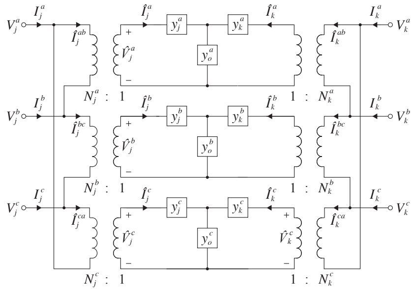
(b) ΔΔ configuration
