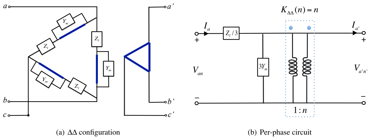
Figure 3.16: Model of three-phase transformers in \Delta\Delta configuration and its per-phase equivalent circuit.
