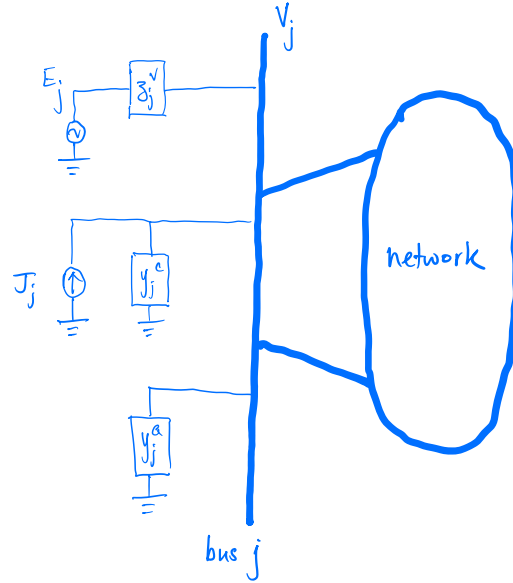
Figure 4.9: Multiple devices connected to the same bus.
