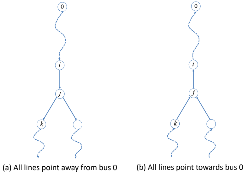
Figure 5.2: Notation for BFM for radial networks.
