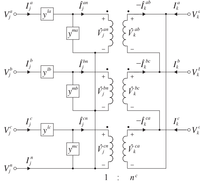
Figure 8.15: Y\Delta -configured transformer.
