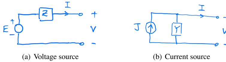
Figure 1.3: A voltage source (E, z) and a current source (J, y) . An ideal voltage source has z = 0 and an ideal current source has y = 0 . (Fig change: Z, Y \rightarrow z, y .)
