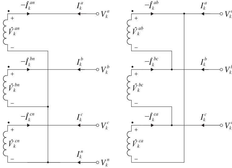
Figure 8.11: Secondary side of a three-phase transformer in Y (left) or \Delta (right) configuration.
