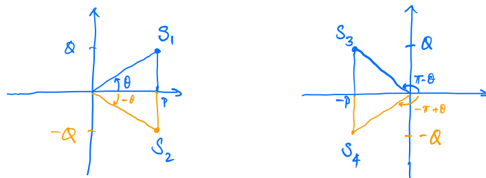
Figure 1.24: Power factor angles \phi and power factor \cos \phi .
