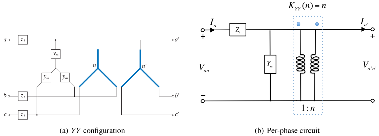
Figure 3.15: Model of three-phase transformers in YY configuration and its per-phase equivalent circuit.
