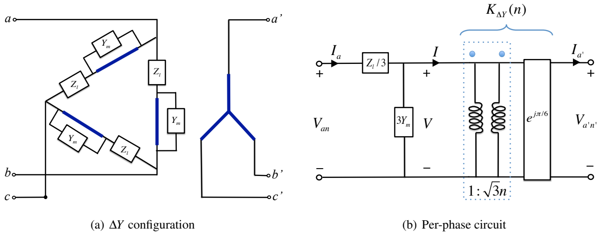
Figure 3.36: Model of three-phase transformers in \Delta Y configuration and its per-phase equivalent circuit.
