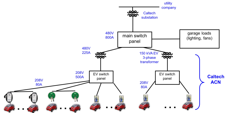
Figure 3.39: Caltech Adaptive Charging Network (ACN) layout.
