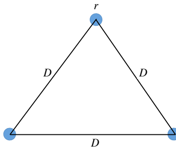
Figure 2.8: Per-meter inductance and capacitance of a symmetric three-phase transmission line in balanced operation.
