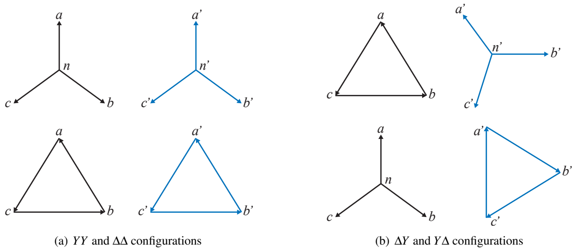
Figure 3.14: Compact representation of ideal three-phase transformers in (a) YY , \Delta\Delta configurations and (b) \Delta Y , Y\Delta configurations. For instance, in the YY configuration, the vertical arrow represents the vector V_{an} in the complex plane. The arrow from b to a (not shown) represents the vector V_{ab} . The parallel lines in the diagram indicate corresponding primary and secondary windings.
