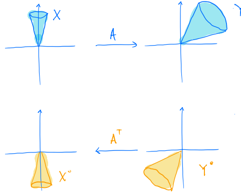
Figure 17.8: Theorem 17.5 when A is nonsingular: linear transformation Y of a convex cone X and their polar cones Y^\circ, X^\circ respectively. By Theorem 17.3, their normal cones at \bar{x} = 0 are N_X(0) = X^\circ and N_Y(0) = Y^\circ respectively. (Changes in figure: (i) X^\circ should have a wider angle. (ii) X^\circ = N_X(0) and Y^\circ = N_Y(0) .)
