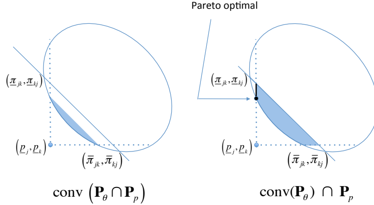
Figure 14.4: \text{conv}(\mathbb{P}_\theta \cap \mathbb{P}_p) \subseteq \text{conv}(\mathbb{P}_\theta) \cap \mathbb{P}_p .
