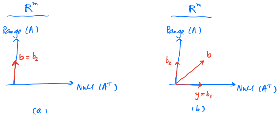
Figure 11.14: Theorem 11.10.2.
