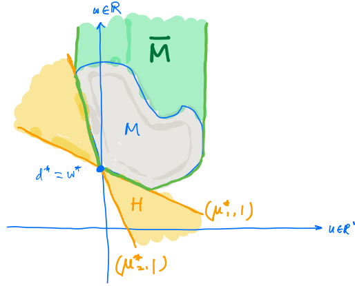
Figure 17.16: Every dual optimal \mu^* \in Q^* defines a hyperplane H that passes through (0, w^*) and separates it from \text{cl}(\bar{M}) . The yellow region shows all the hyperplanes defined by Q^* .
