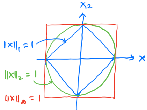
Figure 25.5: The boundaries of unit balls for l_1 , l_2 and l_\infty norms.
