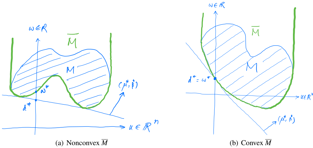
Figure 17.15: The primal and dual problems (17.28) defined by the nonempty set M . Their optimal values are (w^*, d^*) respectively. The normal (\mu^*, \beta^* := 1) of the nonvertical hyperplane attains the dual optimal solution \mu^* , i.e., d(\mu^*) = d^* . (a) Nonzero duality gap d^* < w^* when \bar{M} is not convex. (b) Zero duality gap d^* = w^* when \bar{M} is convex even though M is nonconvex. In both cases, 0 \in \text{ri}(D_{\bar{M}}) which ensures that \beta^* > 0 (nonvertical hyperplane).
