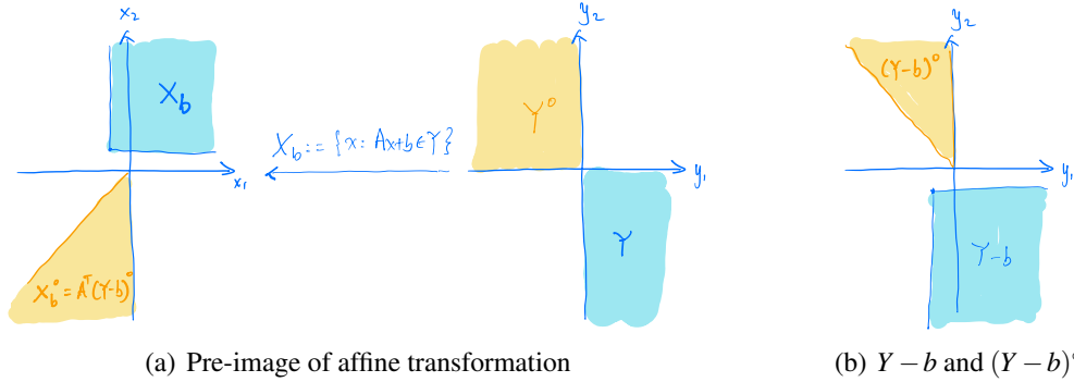
Figure 17.11: Example 17.5: while Y is a cone, X_b is not. According to Theorem 17.8, X_b^\circ = A^\top(Y - b)^\circ and N_{X_b}(\bar{x}) = A^\top N_Y(\bar{y}) .
