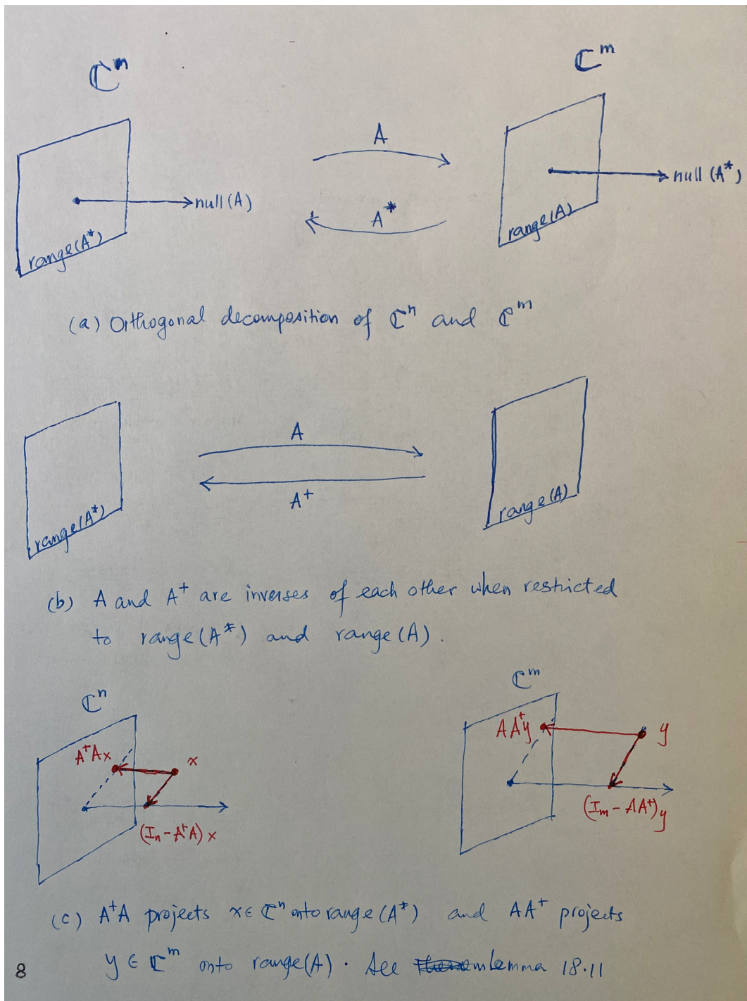
Figure 25.3: (a) Decomposition of \mathbb{C}^n into orthogonal complements \text{null}(A) and \text{range}(A^H) and \mathbb{C}^m into orthogonal complements \text{null}(A^H) and \text{range}(A) . (b) A and A^\dagger are bijective between \text{range}(A^H) and \text{range}(A) inverses of each other. (c) A^\dagger A projects x \in \mathbb{C}^n onto \text{range}(A^H) and AA^\dagger projects y \in \mathbb{C}^m onto \text{range}(A) . See Theorem 25.19.
