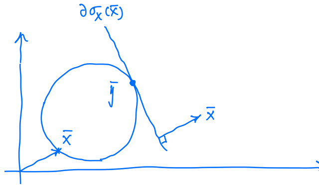
Figure 17.14: For a nonempty closed convex X , \partial\sigma_X(\bar{x}) is a supporting hyperplane of X at \bar{x} .
