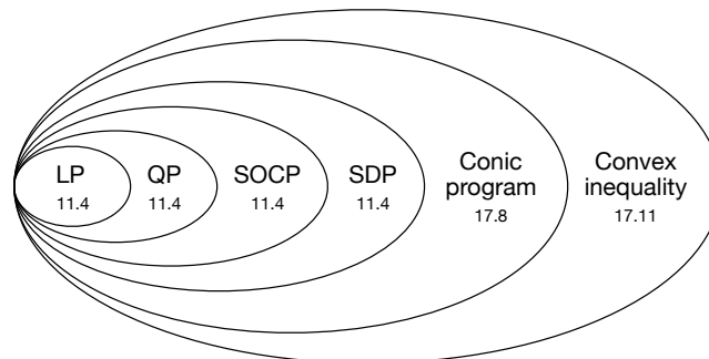
Figure 11.15: Special classes of convex problems studied in this section and Chapter 17.8 using nonsmooth methods. (Doublecheck section references in the figure.)
