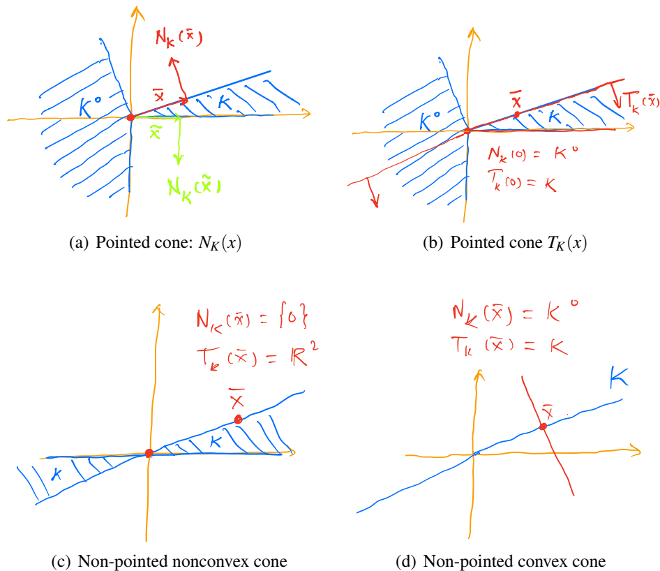
Figure 17.3: Normal and tangent cones of closed cones K \subseteq \mathbb{R}^2 . K^\circ \subseteq \mathbb{R}^2 is the polar cone of K . (a) The normal cones N_K(\bar{x}) and N_K(\tilde{x}) at two boundary points \bar{x} and \tilde{x} are different. At the origin, N_K(0) = K^\circ . At an interior point \bar{x} , N_K(\bar{x}) = \{0\} . (b) The tangent cone T_K(\bar{x}) at a boundary point \bar{x} is a halfspace containing K . At the origin, T_K(0) = K . This satisfies T_K(0) = [N_K(0)]^\circ = [K^\circ]^\circ = K , verifying Proposition 17.2 and Proposition 17.1 since the feasible direction cone \text{cone}(K - 0) = K is a closed convex cone. This is not the case at the boundary point \bar{x} since \text{cone}(K - \bar{x}) is a cone but \text{cone}(K - \bar{x}) \neq K . At an interior point \bar{x} , T_K(\bar{x}) = \mathbb{R}^2 . (c) For this non-pointed nonconvex cone, at all \bar{x} \in K , N_K(\bar{x}) = \{0\} and T_K(\bar{x}) = \mathbb{R}^2 . (d) For this non-pointed convex cone K (which is a hyperplane in \mathbb{R}^2 ), at all \bar{x} \in K , N_K(\bar{x}) = K^\circ is the normal \{y \in \mathbb{R}^n : y^\top x = 0 \forall x \in K\} to the hyperplane K and T_K(\bar{x}) = K .
