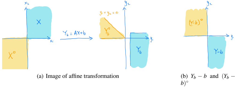
Figure 17.10: Example 17.4: while X is a cone, Y_b is not. According to Theorem 17.7, X^\circ = A^T(Y_b - b)^\circ and N_X(\bar{x}) = A^T N_{Y_b}(\bar{y}) . (Change in figure (a): Change X^\circ to X^\circ = A^T(Y_b - b)^\circ .)
