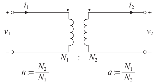
Figure 3.1: Single-phase ideal transformer.
