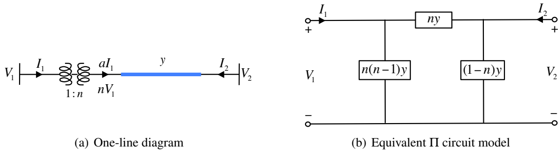
Figure 4.13: An ideal transformer with turns ratio a = n^{-1} followed by a transmission line modeled by a series admittance y .
