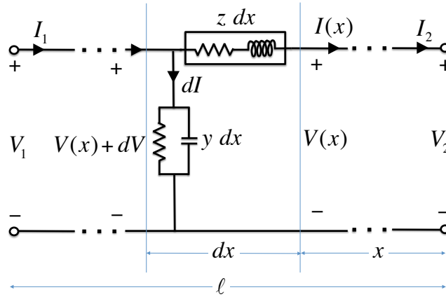
Figure 2.4: Per-phase model of a balanced three-phase line of length \ell with impedance parameters z, y .
