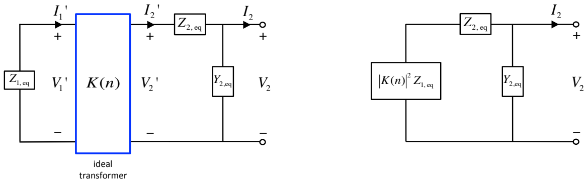
(a) Transformer circuit
