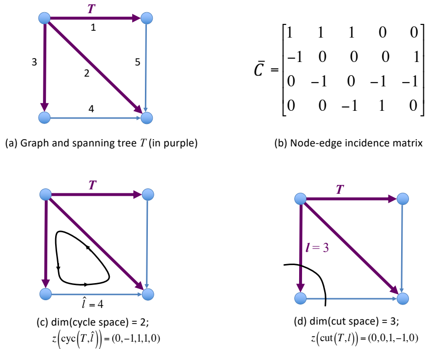
Figure 25.8: (a) A connected graph with a spanning tree T . (b) 4 \times 5 incidence matrix \bar{C} . (c) The cycle subspace \text{null}(\bar{C}) with dimension 2, one for each edge not in the spanning tree T , and an example basis vector z(\text{cyc}(T, l)) \in \text{null}(\bar{C}) . (d) The cut subspace \text{range}(\bar{C}^T) with dimension 3, one for each edge in T , and an example basis vector z(\text{cut}(T, l)) \in \text{range}(\bar{C}^T) . The examples z(\text{cyc}(T, l)) and z(\text{cut}(T, l)) are indeed orthogonal.
