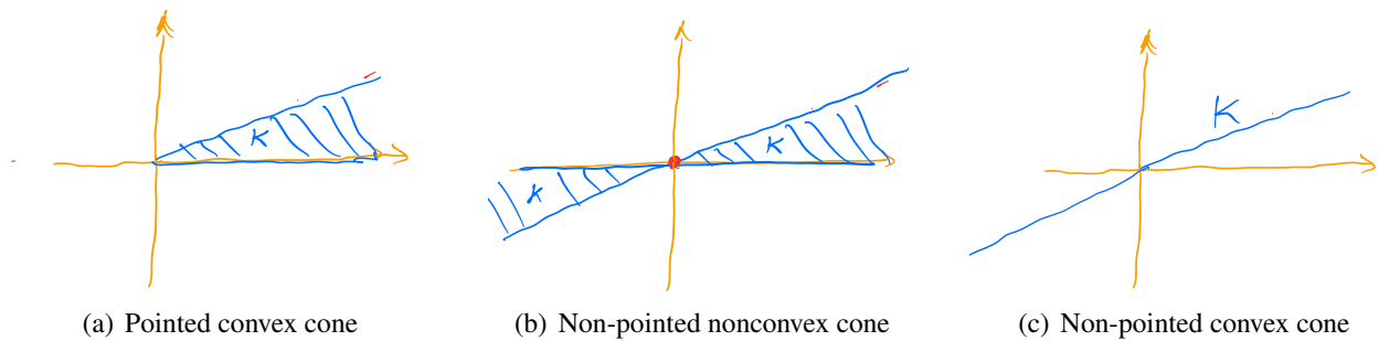
Figure 11.2: Cones and their affine hulls. (a) A pointed convex cone K . It is not a subspace; its affine hull \text{aff}(K) = \mathbb{R}^2 . (b) A non-pointed nonconvex cone K . It is not a subspace; its affine hull \text{aff}(K) = \mathbb{R}^2 . (c) A non-pointed convex cone K which is a subspace. Hence \text{aff}(K) = K .
