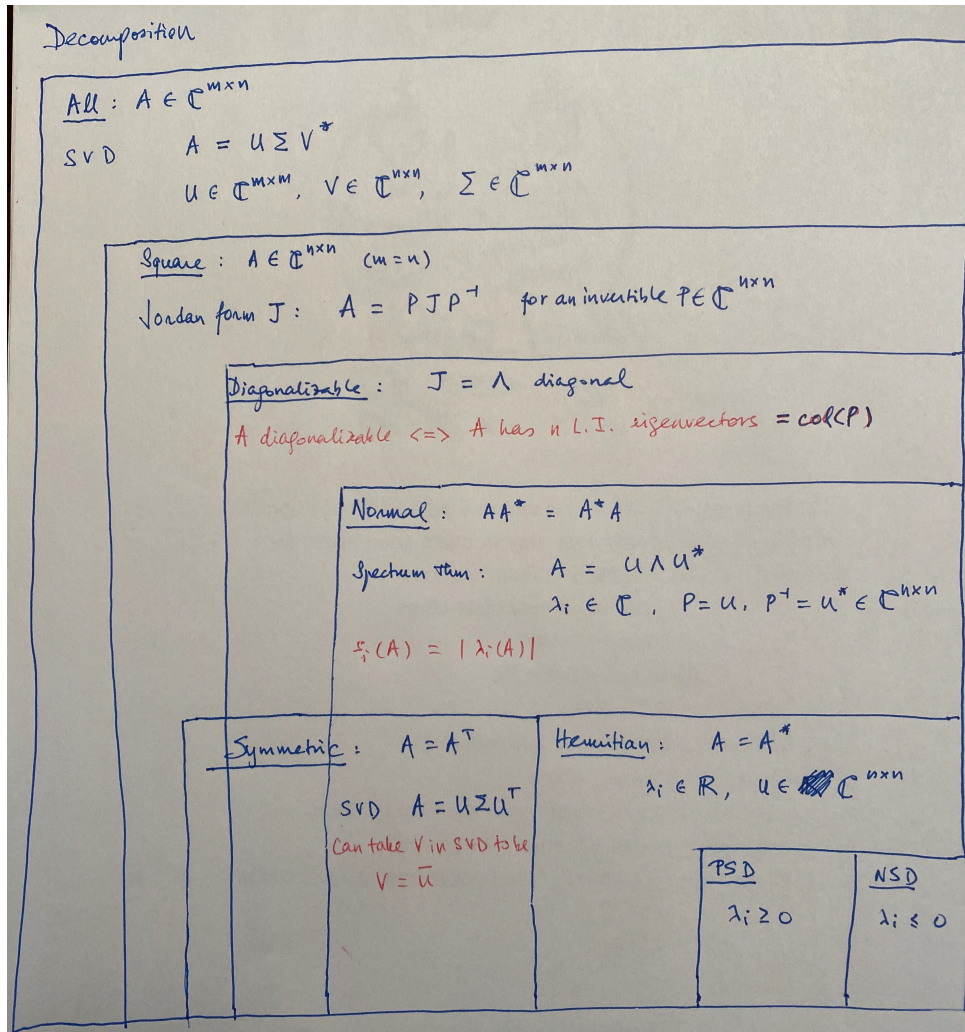
Figure 25.2: Matrix decompositions. Correction: For complex symmetric A , the unitary factor U in Takagi factorization is generally not eigenvectors of AA^H .
