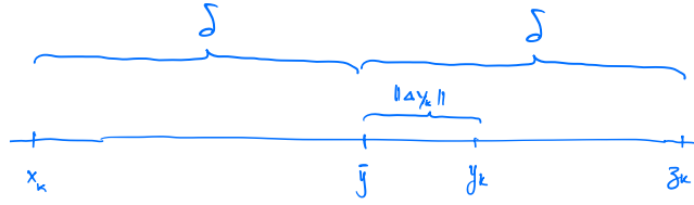
Figure 11.9: Proof of Lemma 11.6: Construction of (x_k, z_k) from \bar{y} and y_k .
