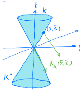
Figure 17.12: Theorem 17.9: The normal cone N_K((\bar{x}, \bar{s})) is the line segment on the boundary of the lower cone K^\circ in the direction of \bar{x} .
