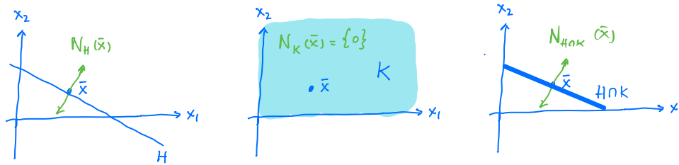
(a) At a relative interior point \bar{x} of H \cap K .
