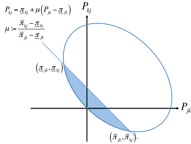
Figure 14.5: The set \text{conv}(\mathbb{P}_\theta) is the intersection of the ellipse, including its interior, and a half-space.
