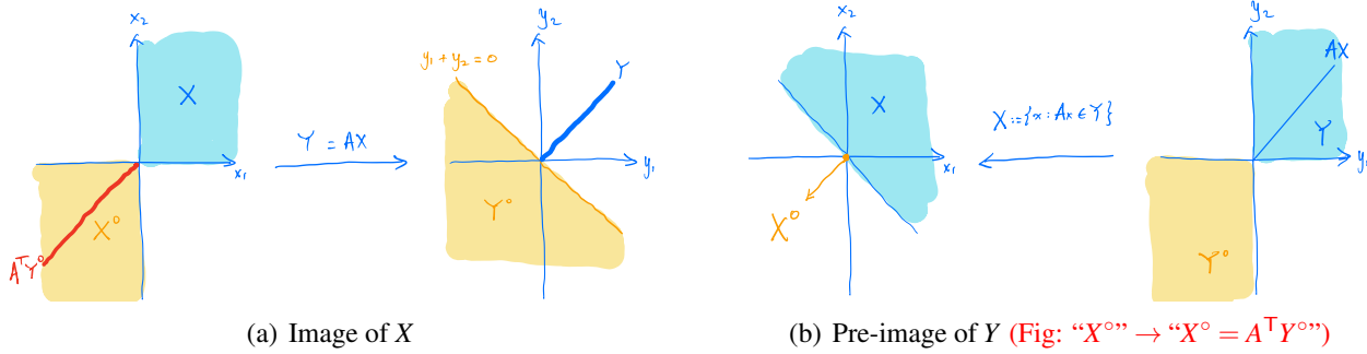
Figure 17.9: Example 17.3. Since A is singular, (a) A^T Y^\circ \subsetneq X^\circ ; (b) AX \subsetneq Y .
