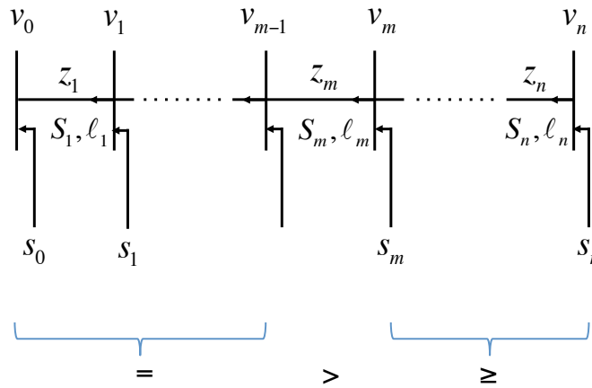
Figure 15.3: Linear network and notations. Line m in the proof is the line closest to bus 0 where the inequality in (15.29) is strict, i.e., (15.29) holds with equality at lines j = 1, \dots, m - 1 , strict inequality at line m , and inequality at lines j = m + 1, \dots, N .
