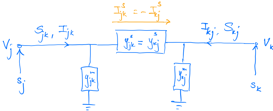
Figure 5.1: Line model under assumption C5.1.
