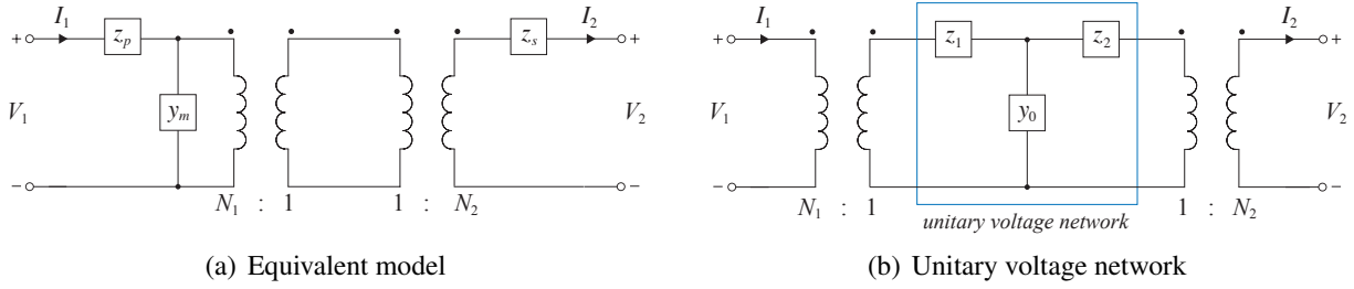
Figure 3.8: Models of nonideal transformer with unitary voltage network.
