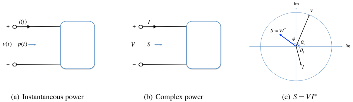
Figure 1.23: Definition of power
