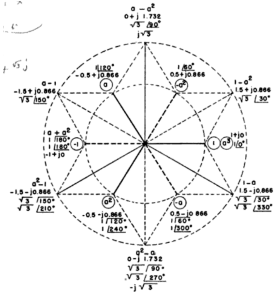
FIG. 3. Graphical representation of functions of the operator a .
