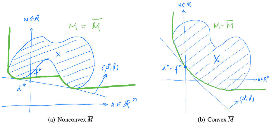
Figure 17.17: The (u, w) space is defined by the feasible set X which defines M = \overline{M} (cf. M in Figure 17.15). (Figure change: \mathbb{R}^n \rightarrow \mathbb{R}^l .)
