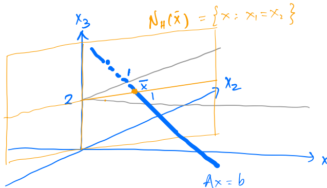
Figure 17.5: Example 17.2: normal cone N_{H_1}(\bar{x}) of the hyperplane H_1 . (Fig change: (i) H \rightarrow H_1 . (ii) Add subfigure for H_2 ?)
