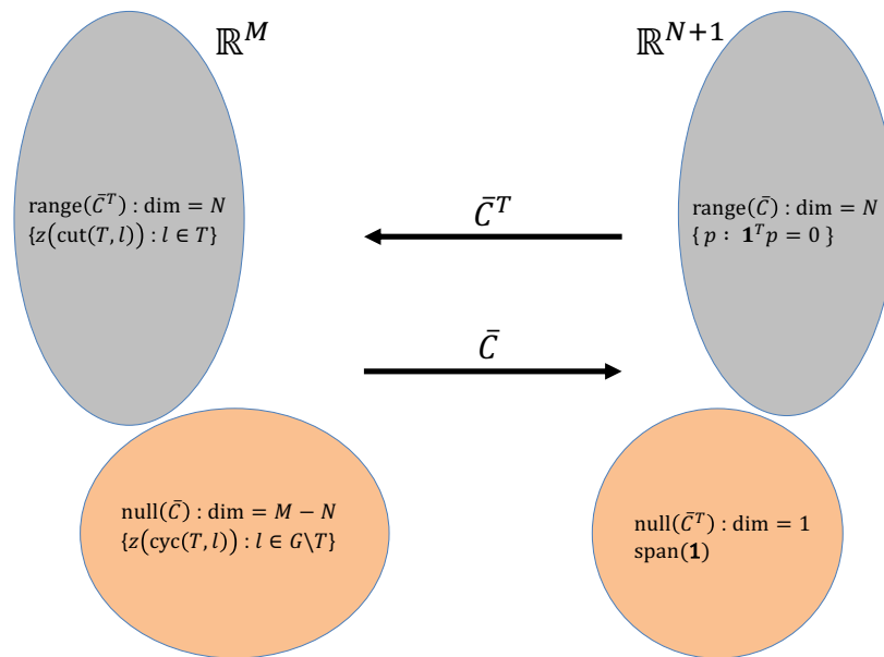
Figure 25.7: The edge space of a connected graph G is \mathbb{R}^M = \text{null}(\bar{C}) \oplus \text{range}(\bar{C}^T) . The cycle subspace \text{null}(\bar{C}) has dimension M - N with a basis \{z(\text{cyc}(T, l)) : l \in G \setminus T\} , and the cut subspace \text{range}(\bar{C}^T) has dimension N with a basis \{z(\text{cut}(T, l)) : l \in T\} . The vertex space is \mathbb{R}^{N+1} = \text{null}(\bar{C}^T) \oplus \text{range}(\bar{C}) with dimension N and 1.
