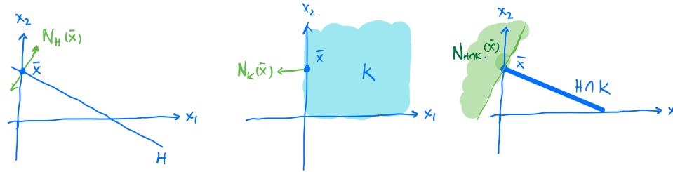
(b) At a relative boundary point \bar{x} of H \cap K
