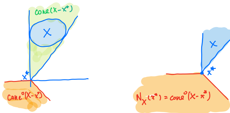
Figure 17.6: Geometric interpretation of Theorem 11.8. (a) When x^* \in \text{cl}(X) \setminus \text{int}(X) , \hat{x}^* = x^* and \text{cone}^\circ(\text{cl}(X) - x^*) = N_{\text{cl}(X)}(\hat{x}^*) . (b) When x^* \notin \text{cl}(X) , \text{cone}^\circ(\text{cl}(X) - x^*) \supseteq N_{\text{cl}(X)}(\hat{x}^*) but these sets may not be equal. (Fig change: Change into 2 subfigures and switch their order. ALL X should be \text{cl}(X) in figure.)
