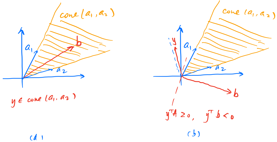
Figure 11.13: Theorem 11.10.1.
