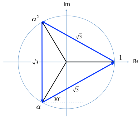
Figure 1.10: Phase shift \alpha := e^{-i2\pi/3} in Theorem 1.2.
