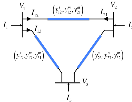
Figure 4.8: Three-bus network of Example 4.3.
