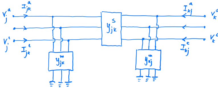
Figure 8.2: A three-wire line characterized by 3 \times 3 series and shunt admittance matrices (y_{jk}^s, y_{jk}^m, y_{kj}^m) .
