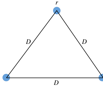
Figure 2.2: Per-meter inductance and capacitance of a symmetric three-phase transmission line in balanced operation.
