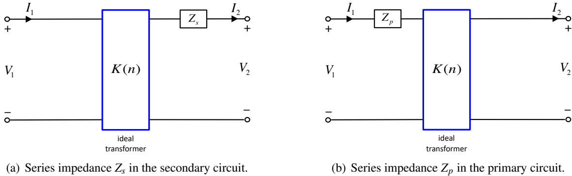
Figure 3.19: Referring series impedance in the secondary to the primary.
