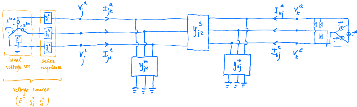
Figure 8.7: A voltage source connected to a current source through the line in Figure 8.2.
