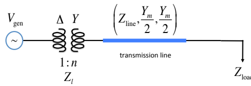
Figure 3.38: A three-phase generator in \Delta configuration connected to a three-phase \Delta Y transformer and then to a three-phase load in Y configuration through a three-phase AC transmission line.
