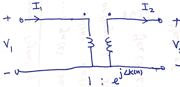
Figure 3.32: Normalization when connection-induced phase shifts cannot be ignored.
