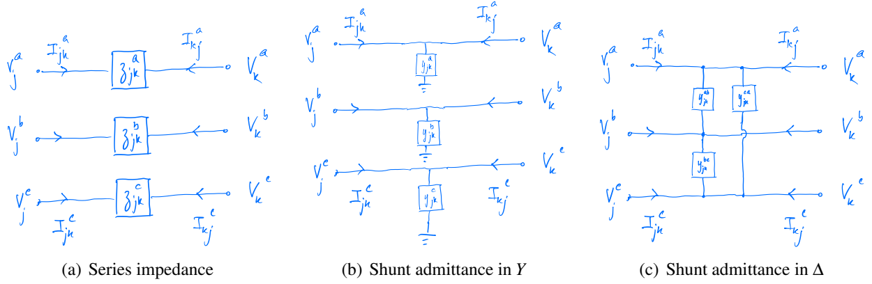
Figure 8.4: Special three-wire lines characterized by (8.10).
