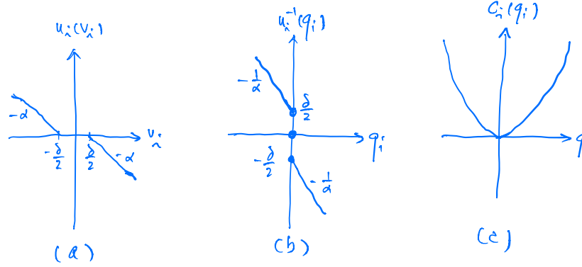
Figure 5.6: (a) The piecewise linear control function u_j(v_j) , (b) its inverse u_j^{-1}(q_j) , and (c) the implied cost function c_j(q_j) .
