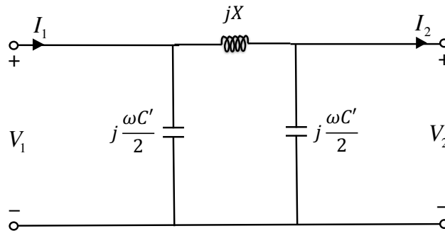
Figure 2.6: \Pi circuit model for a lossless line with length \ell < \pi/\beta .
