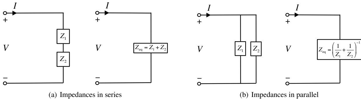
Figure 3.22: (a) Thévenin equivalent Z_{eq} of two impedances Z_1, Z_2 in series. (b) Thévenin equivalent Z_{eq} of two impedances Z_1, Z_2 in parallel.
