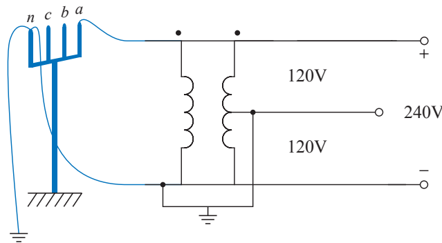
Figure 3.7: A common single-phase distribution transformer in the US.
