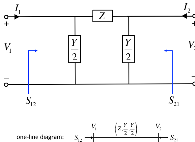
Figure 2.9: Two buses connected by a transmission line.
