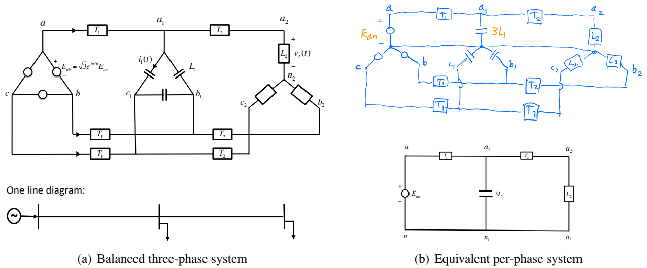
Figure 1.19: Balanced three-phase system and its per-phase equivalent circuit. The balanced three-phase loads have admittances l_1 and l_2 , and the transmission lines have admittances t_1 and t_2 . (Fig change: T \rightarrow t , L \rightarrow l .)
