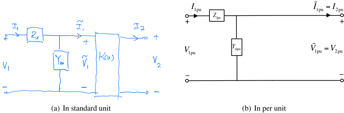
Figure 3.29: Per-phase equivalent circuit of balanced three-phase transformers with gain K(n) .
