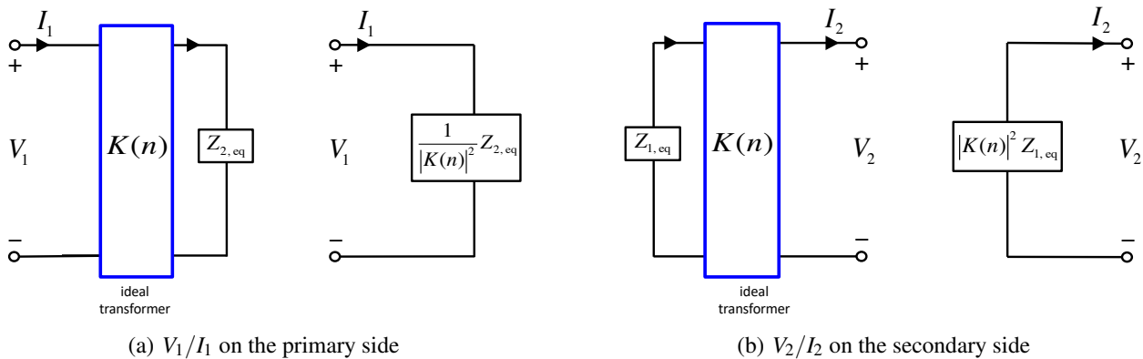
Figure 3.23: Driving-point impedances
