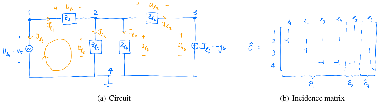
Figure 1.4: A circuit represented as a directed graph where each link l is either an impedance z_l , a voltage source U_l , or a current source J_l . The voltage source U_{l_5} = u_5 and current source J_{l_6} = -j_6 are given. Its incidence matrix \hat{C} is partitioned into \hat{C}_1 corresponding to the impedances, \hat{C}_2 corresponding to the voltage source, and \hat{C}_3 corresponding to the current source. (Fig change: Z_{l_1}, Z_{l_2}, \dots \rightarrow z_{l_1}, z_{l_2}, \dots )
