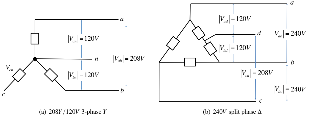
Figure 1.20: Common distribution transformer configurations.
