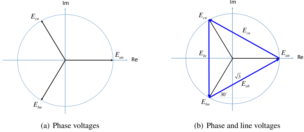
Figure 1.12: A balanced three-phase source in Y configuration. (a) Its phase voltage (vector) E^Y := (E^{an}, E^{bn}, E^{cn}) is a balanced vector. (b) Its line voltage E^{\text{line}} = \Gamma E^Y = (1 - \alpha)E^Y .
