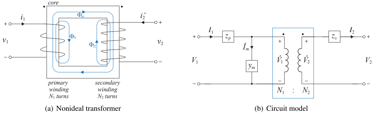
Figure 3.2: Single-phase nonideal transformer. The dashed box represents an ideal transformer with a := N_1/N_2 . (Megan: \hat{U}_1 \rightarrow \hat{V}_1 , \hat{U}_2 \rightarrow \hat{V}_2 .)
