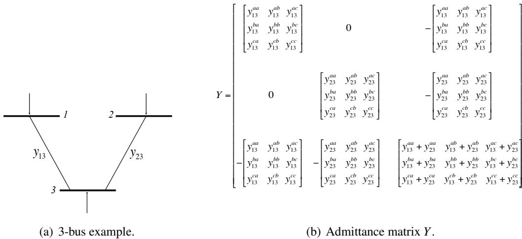
Figure 9.2: The admittance matrix Y for a 3-terminal network with no shunt admittances.
