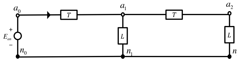
Figure 1.15: The per-phase equivalent circuit of the balanced system in Figure 1.14 in Y configuration. (Fig change: T \rightarrow t , L \rightarrow l , and Y \rightarrow y .)
