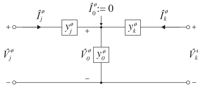
Figure 8.18: Unitary voltage network in each phase \phi of a three-phase transformer.
