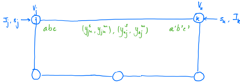
Figure 9.1: A model of three-phase system.
