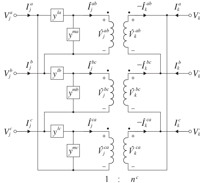
Figure 8.13: \Delta\Delta -configured transformer.
