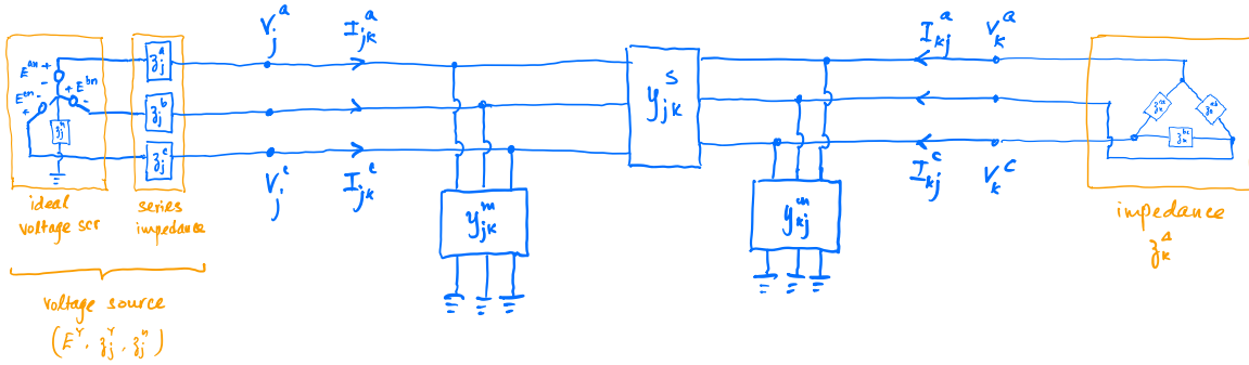
Figure 8.3: A voltage source connected to an impedance load through the line in Figure 8.2.
