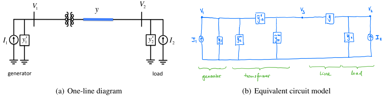
Figure 4.6: Generator, transformer, transmission line and load.
