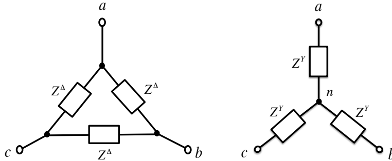
Figure 1.18: \Delta - Y transformation of balanced loads: Z^Y = Z^\Delta/3 . (Fig change: Z \rightarrow z .)
