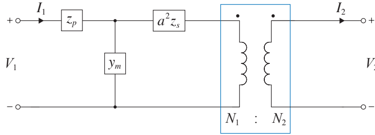
Figure 3.4: T equivalent circuit.
