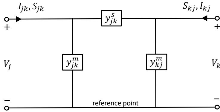
Figure 4.1: \Pi circuit model of a single-phase line.
