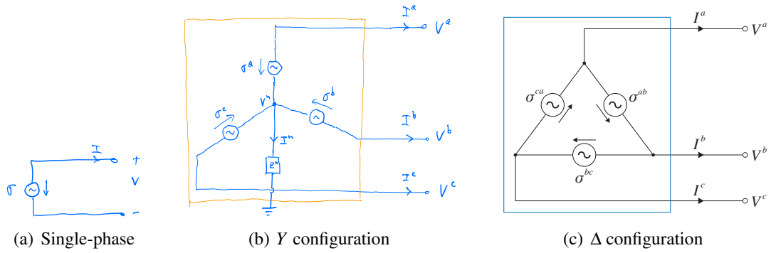
Figure 7.11: Comparison of single-phase and three-phase power sources.
