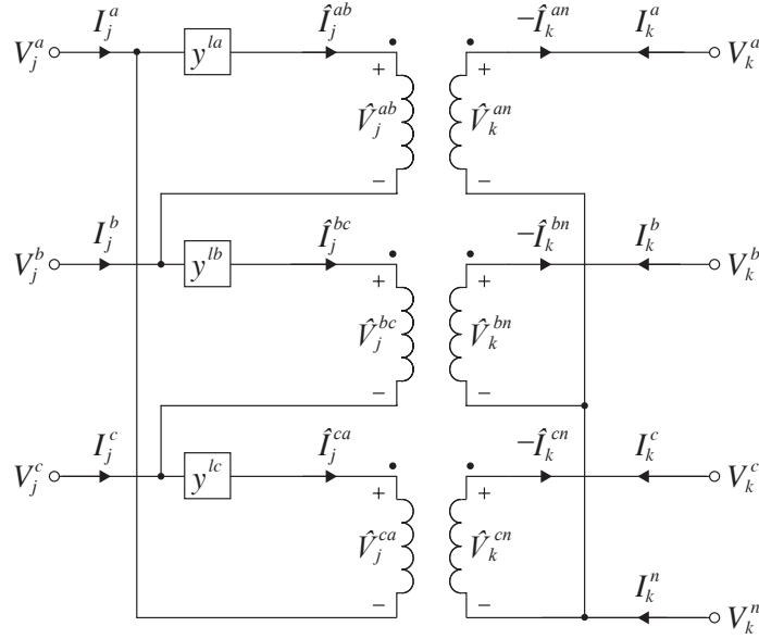
Figure 8.21: \Delta Y -configured transformer with zero shunt admittances.
