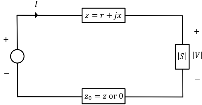
Figure 1.26: A system that delivers power |S| to a load at voltage |V| . The distance between the generation and the load is d . The line has an impedance z := r + jx per unit length.
