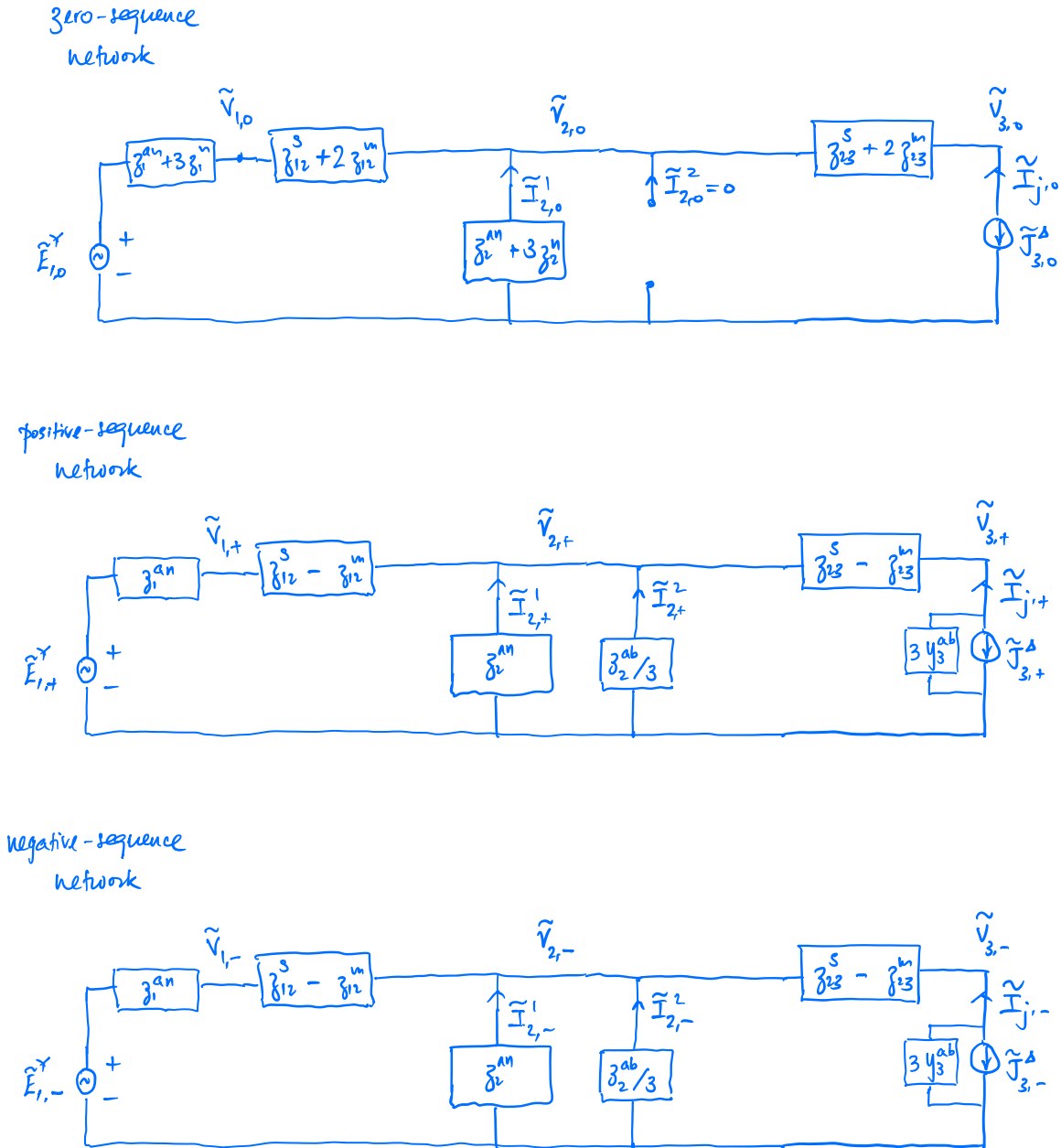
Figure 9.10: Example 9.13: Circuit models of sequence networks.
