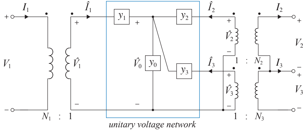
Figure 3.10: Single-phase split-phase transformer.
