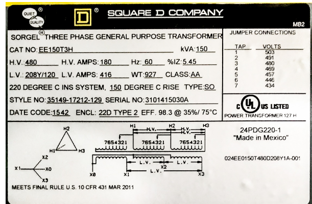
(b) Transformer ratings
