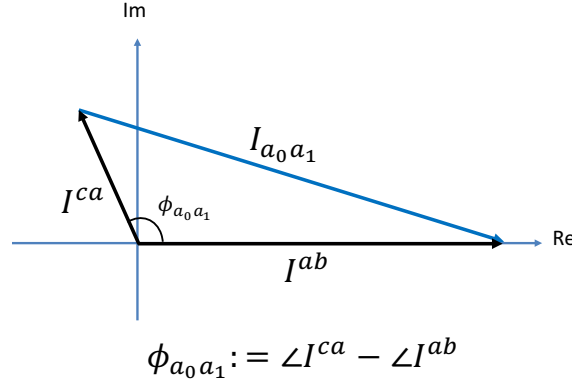
Figure 1.22: I^{a_0 a_1} = I^{ab} - I^{ca} . Hence by the cosine rule |I^{a_0 a_1}|^2 = |I^{ab}|^2 + |I^{ca}|^2 - 2 |I^{ab}| |I^{ca}| \cos \phi where \phi_{a_0 a_1} := \angle I^{ca} - \angle I^{ab} is the angle between I^{ab} and I^{ca} .
