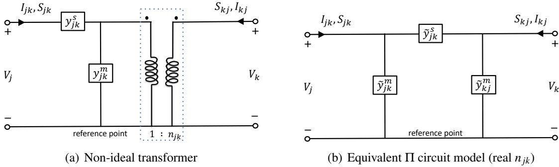
Figure 4.2: Single-phase transformer.
