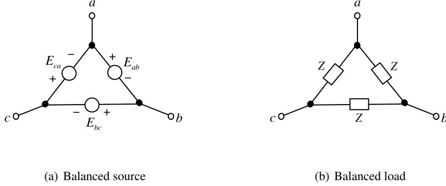
Figure 1.16: Balanced three-phase (a) voltage source E^\Delta and (b) impedance z^\Delta in \Delta configuration. (Fig change: Z \rightarrow z .)
