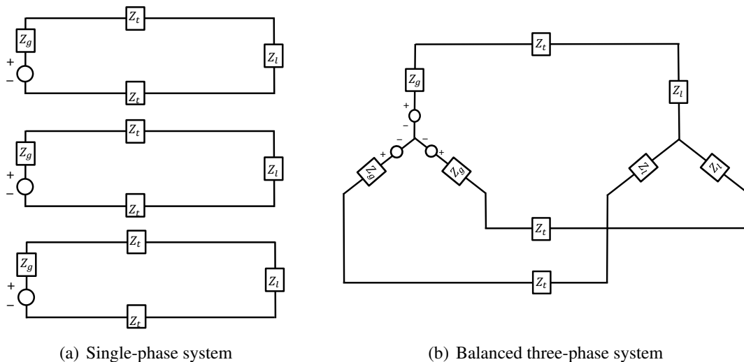
Figure 1.7: A single-phase system and a balanced three-phase system that transfer power from generators through transmission lines to loads. (Fig change: Z \rightarrow z .)
