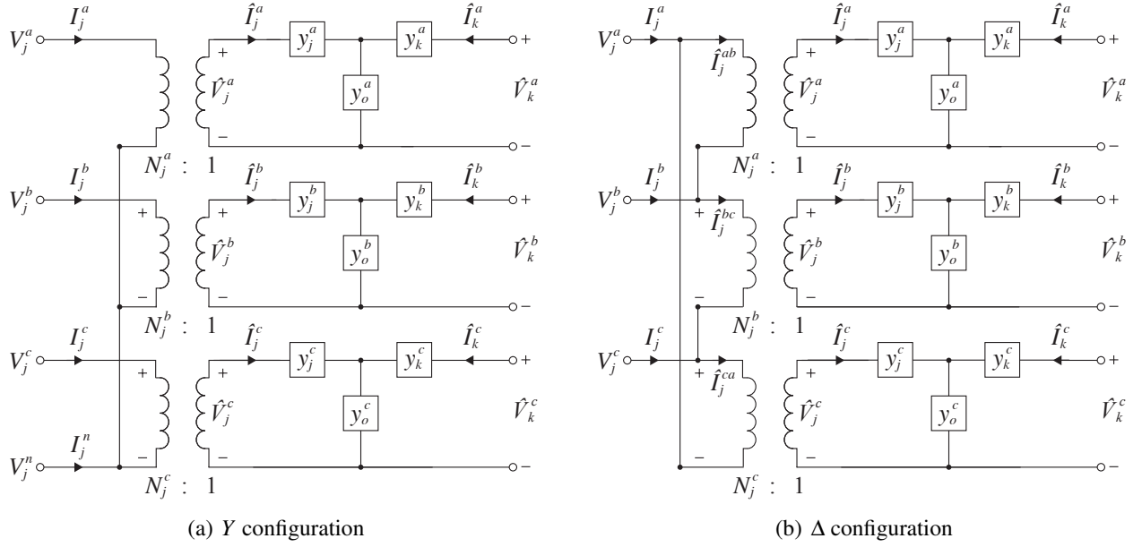
Figure 8.19: Primary side of a three-phase transformer with unitary voltage networks.
