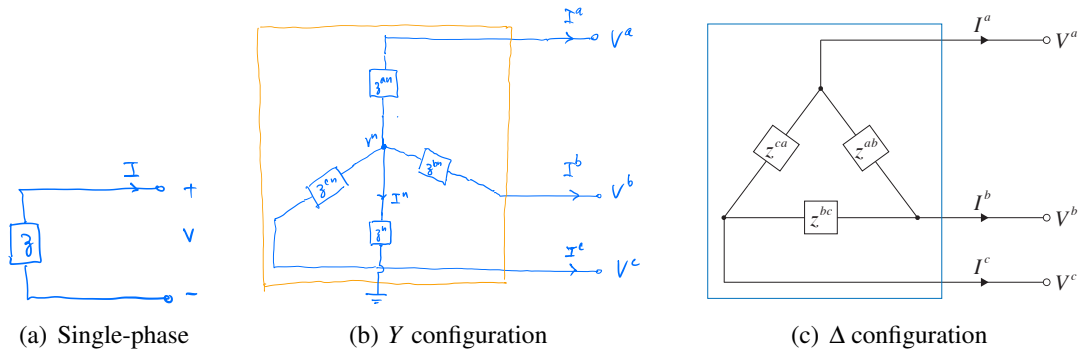
Figure 7.12: Comparison of single-phase and three-phase impedances.
