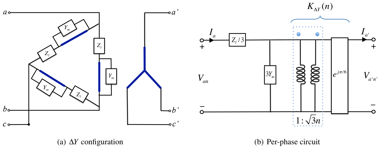
Figure 3.17: Model of three-phase transformers in \Delta Y configuration and its per-phase equivalent circuit.
