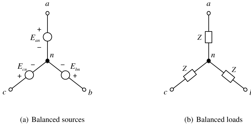
Figure 1.11: Balanced three-phase (a) voltage source E^Y and (b) impedance z^Y := \text{diag}(z, z, z) in Y configuration. (Fig change: Z \rightarrow z .)
