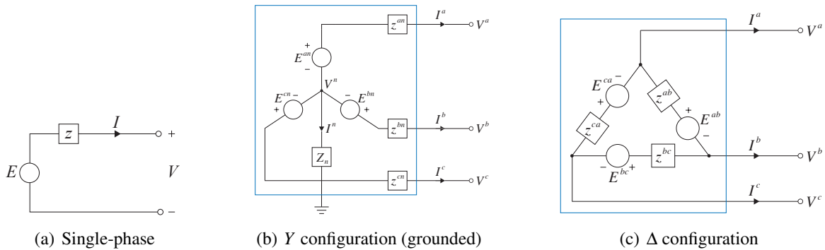
Figure 7.9: Comparison of single-phase and three-phase voltage sources.
