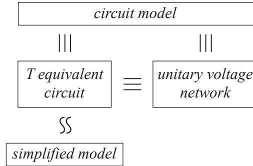
Figure 3.3: Relation between different circuit models of transformers.
