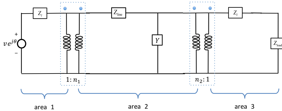
Figure 3.30: Single-phase system for Example 3.8 with a rated voltage magnitude of v in V and a rated apparent power of s in VA.
