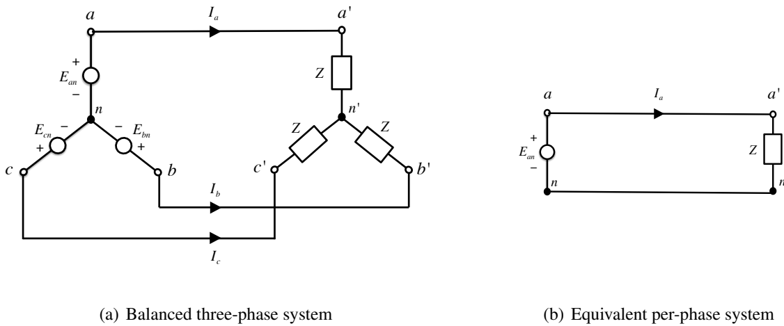
Figure 1.13: Balanced three-phase source and load in Y configuration and its per-phase model. (Fig change: Z \rightarrow z .)
