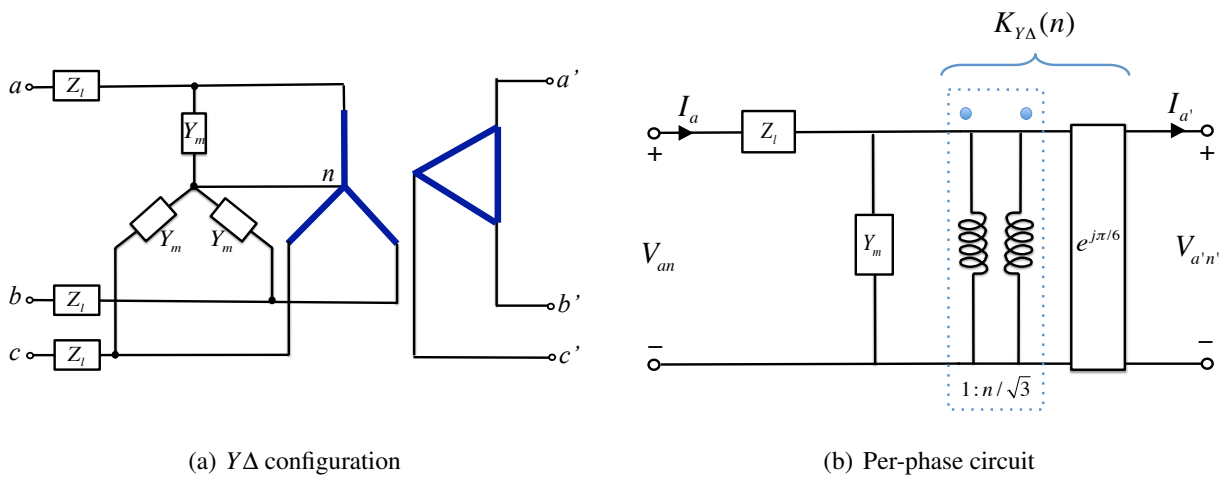
Figure 3.18: Model of three-phase transformers in Y\Delta configuration and its per-phase equivalent circuit.
