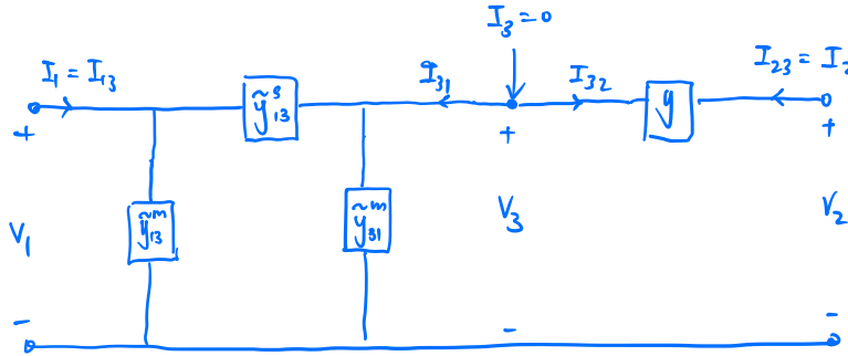
Figure 4.5: \Pi circuit model of the system in Figure 4.4.
