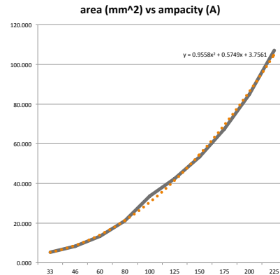
(b) AWG plot
