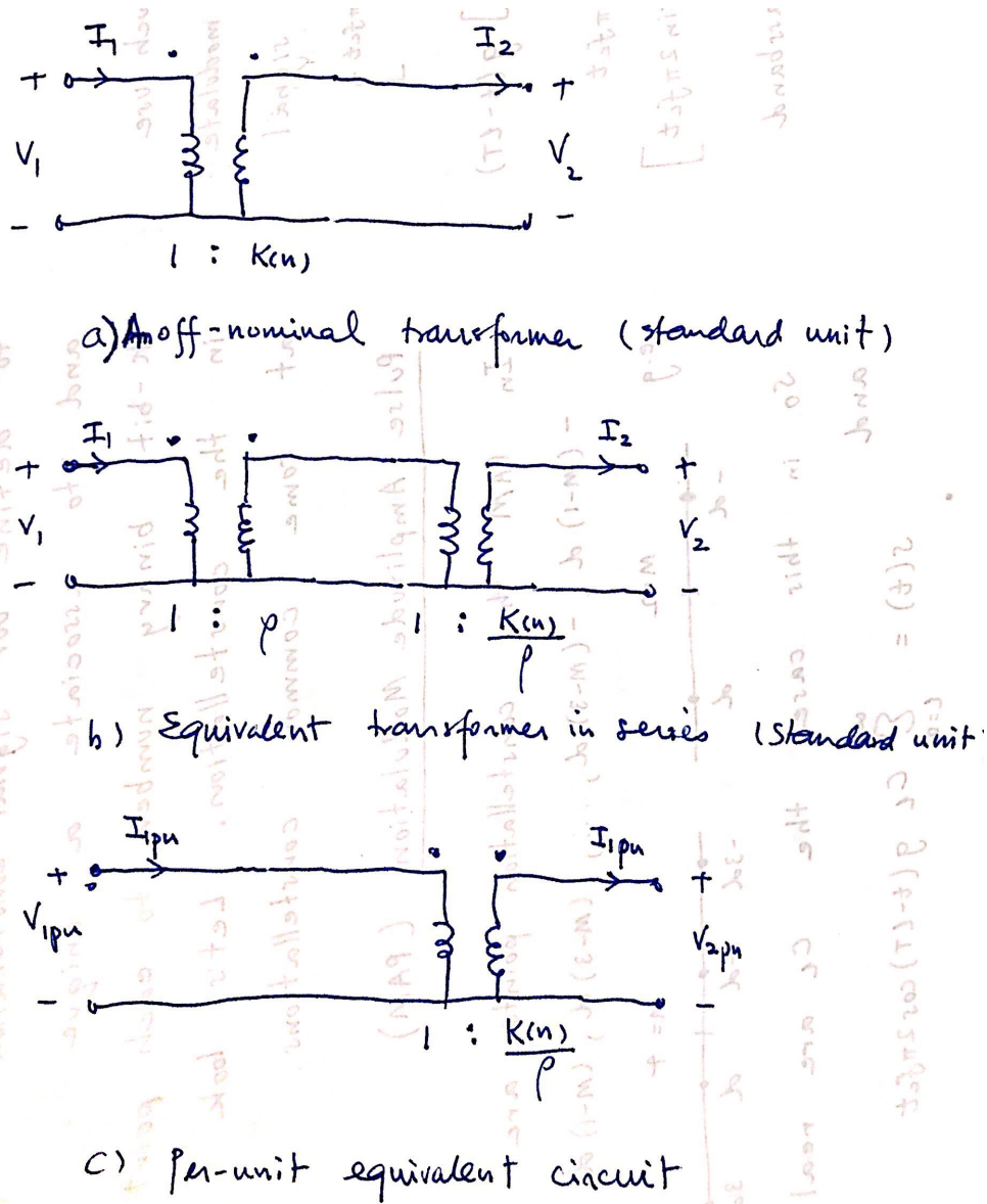
Figure 3.31: Normalization of an off-nominal transformer.
