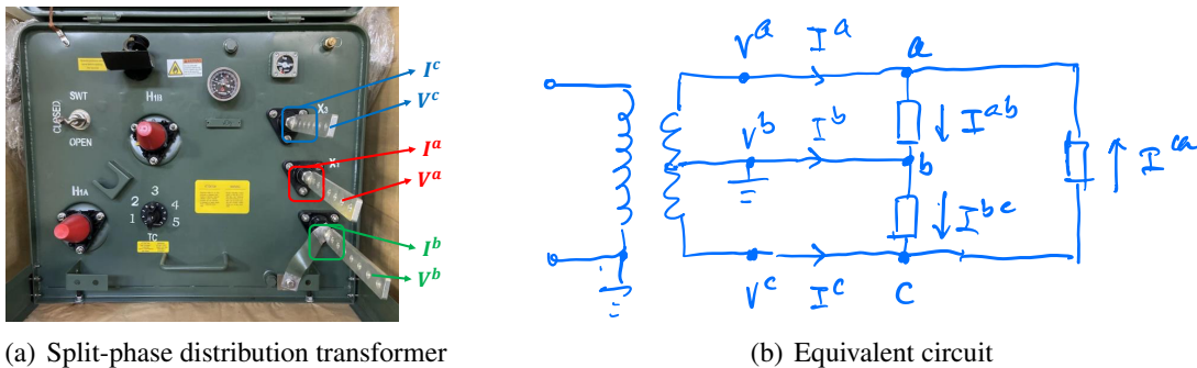
Figure 7.4: Typical distribution transformer and the equivalent circuit of the Southern California system supplying 8 houses arranged in \Delta configuration.
