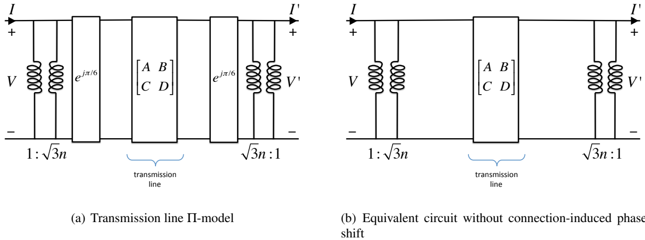
Figure 3.27: \Pi -model of transmission line in place of the series impedance Z_{\text{line}} model in Figure 3.26(b).
