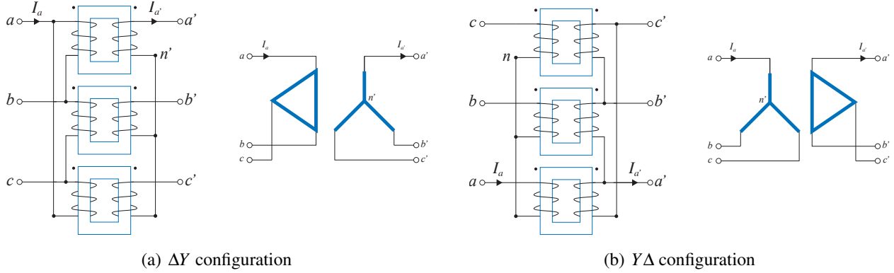
Figure 3.13: Ideal three-phase transformers in \Delta Y and Y\Delta configurations. The parallel lines in the schematic diagram indicate corresponding primary and secondary windings. Note the wiring of the Y\Delta configuration.
