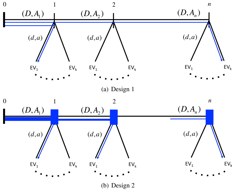
Figure 3.42: Caltech ACN network design.
