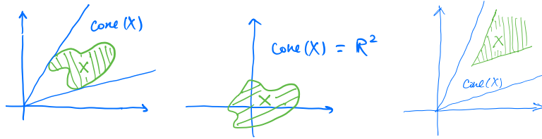
Figure 11.3: Cones \text{cone}(X) generated by X \subseteq \mathbb{R}^n .
