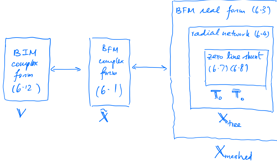
Figure 5.3: Equivalence of BFM and BIM (the model \mathbb{T}_0 defined by (5.7) is the original DistFlow model).
