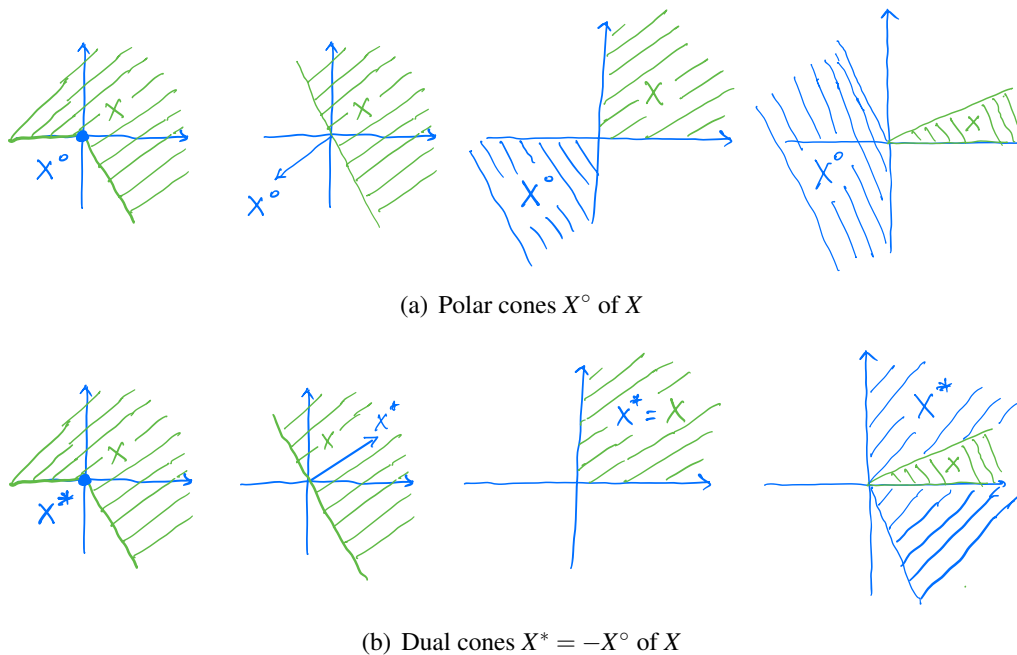
Figure 17.1: Polar cones and dual cones of X \subseteq \mathbb{R}^n . For the leftmost set X which is nonconvex, both its polar cone and dual cone contain only the origin. The other three sets X are closed convex cones and therefore (X^\circ)^\circ = X .
