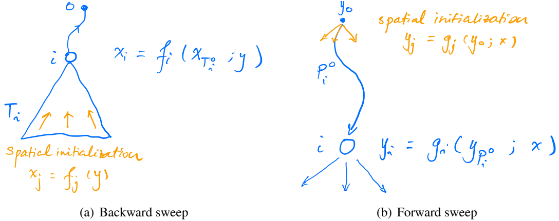
Figure 5.4: General backward forward sweep
