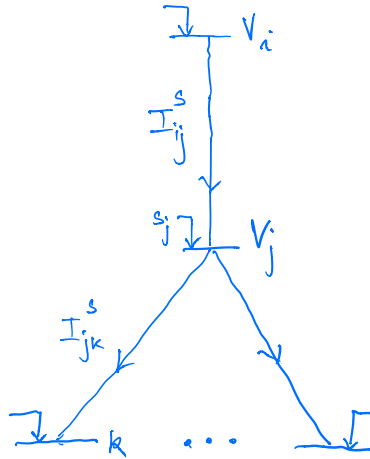
Figure 5.5: Recursive structure of power flow equations (5.25).
