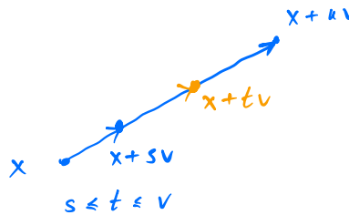
Figure 11.7: Proof of Theorem 11.4.1.
