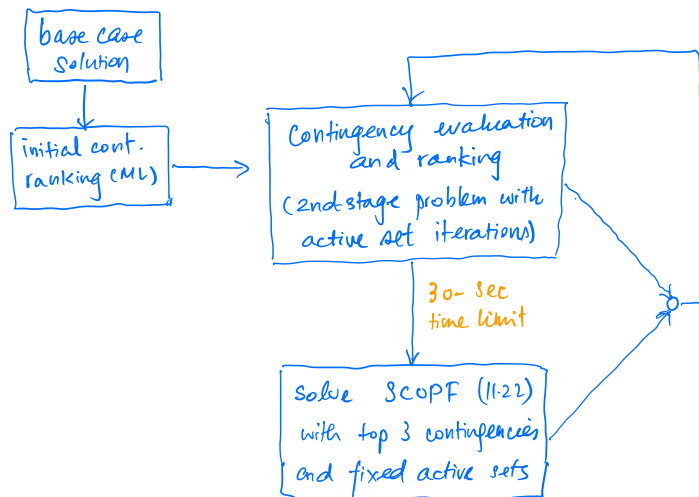
Figure 13.1: Overall algorithm of [130] to compute the first-stage optimal solution x_0^* .
