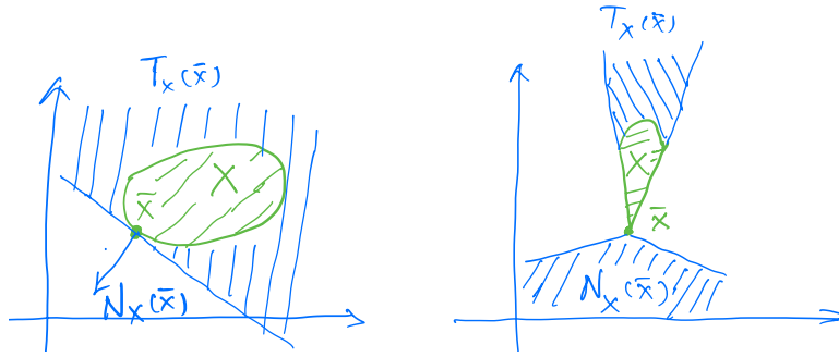
Figure 17.4: The tangent cones T_X(\bar{x}) = \text{cl}(\text{cone}(X - \bar{x})) and the normal cones N_X(\bar{x}) = \text{cone}^\circ(X - \bar{x}) of X at \bar{x} . At \bar{x} where the boundary of X is “smooth”, the left panel illustrates the importance of “cl” in the definition of T_X(\bar{x}) and why N_X(\bar{x}) is a singleton.
