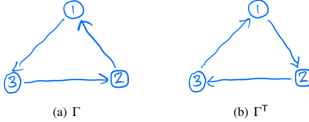
Figure 1.9: Directed graphs of which \Gamma and \Gamma^T are incidence matrices.
