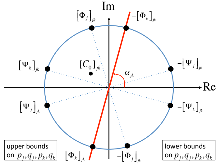
Figure 14.2: Condition C14.2' for OPF on a line (j, k) \in E . The quantities ([\Phi_j]_{jk}, [\Phi_k]_{jk}, [\Psi_j]_{jk}, [\Psi_k]_{jk}) on the left-half plane correspond to finite upper bounds on (p_j, p_k, q_j, q_k) in (14.19a)(14.19b); (-[\Phi_j]_{jk}, -[\Phi_k]_{jk}, -[\Psi_j]_{jk}, -[\Psi_k]_{jk}) on the right-half plane correspond to finite lower bounds on (p_j, p_k, q_j, q_k) .
