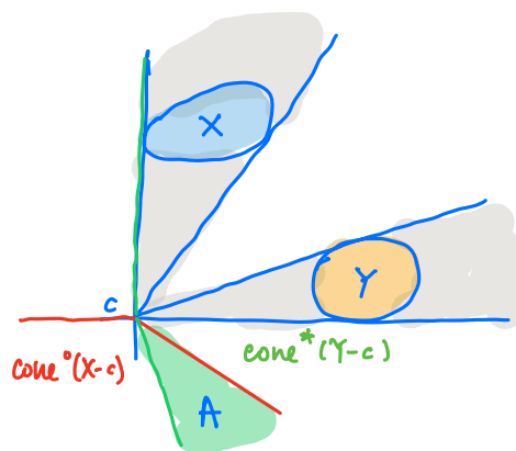
Figure 17.7: Geometric interpretation of Theorem 11.9: If X and Y are disjoint and convex then there exists a possibly new origin z such that the intersection A := \text{cone}^\circ(\text{cl}(X) - z) \cap \text{cone}^*(\text{cl}(Y) - z) is nonempty. (ALL X, Y should be \text{cl}(X) and \text{cl}(Y) respectively in figure. Change c to z .)
