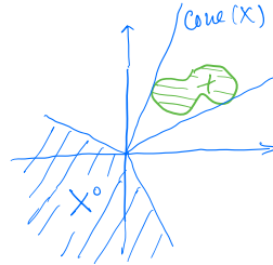
Figure 17.2: Polar cone X^\circ = \text{cone}^\circ(X) according to Proposition 17.1.
