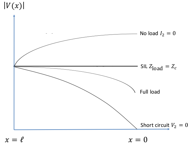
Figure 2.7: Voltage magnitude |V(x)| on a lossless line.
