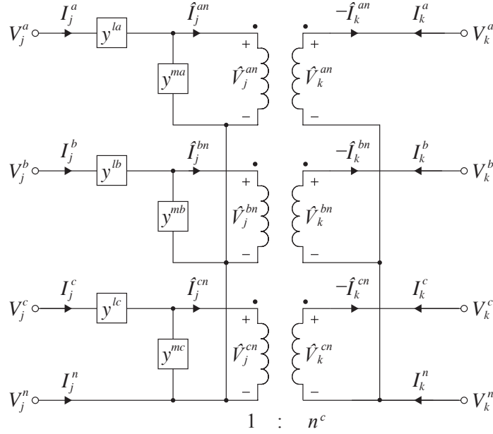
Figure 8.12: YY-configured transformer.
