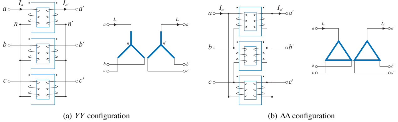
Figure 3.12: Ideal three-phase transformers in YY and ΔΔ configurations. The parallel lines in the schematic diagram indicate corresponding primary and secondary windings.
