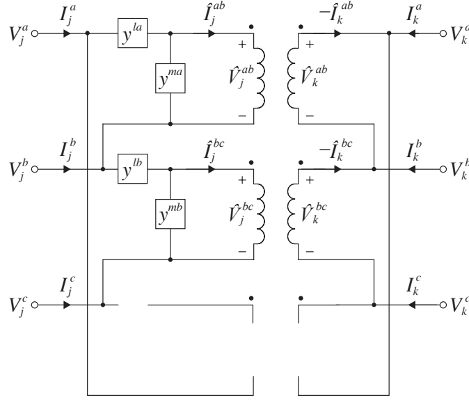
Figure 8.16: Open \Delta\Delta -configured transformer.
