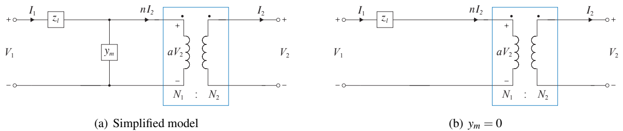
Figure 3.5: (a) Simplified model of nonideal transformer including power losses, leakage flux and finite permeability of magnetic core. (b) Simplified model assuming infinite permeability.
