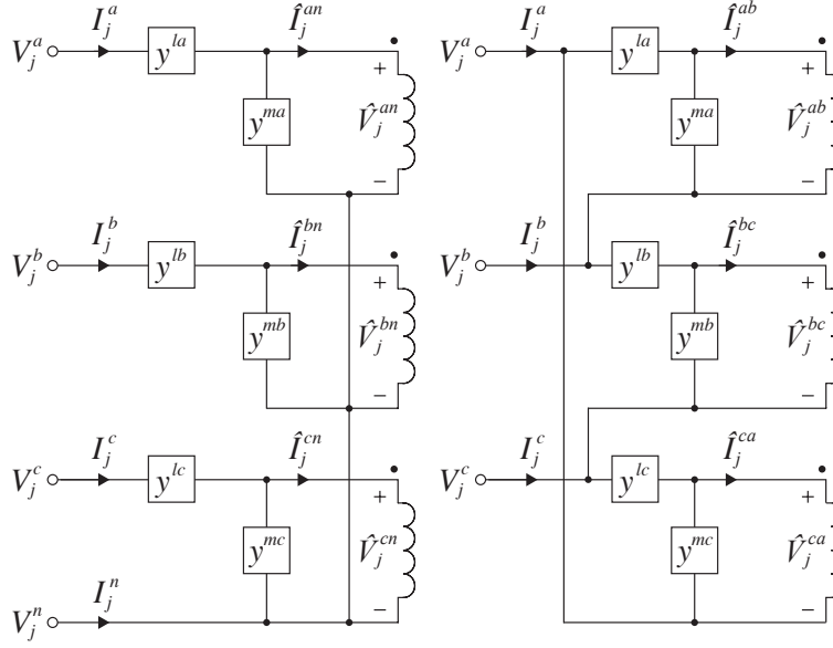
Figure 8.10: Primary side of a three-phase transformer in Y (left) or \Delta (right) configuration. (Add shunt admittance y^m ; see Figures 8.21, 8.22.)
