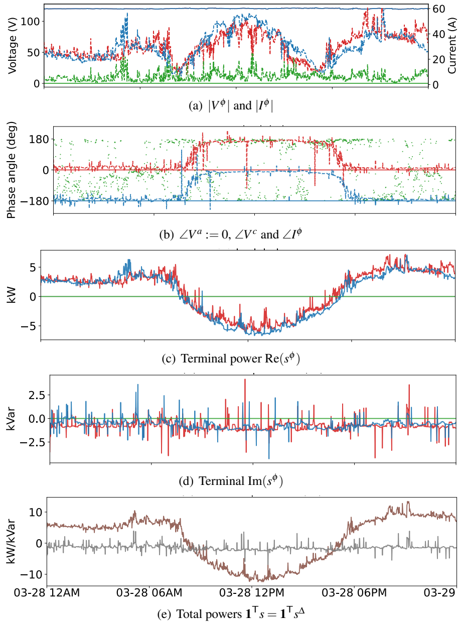
Figure 7.5: Voltage, current and power behavior. (a)(b)(c)(d) Solid lines: voltages, dashed lines: currents. Red: phase a , green: phase b , blue: phase c . (e) Brown: real (kW), grey: imaginary (kVar).
