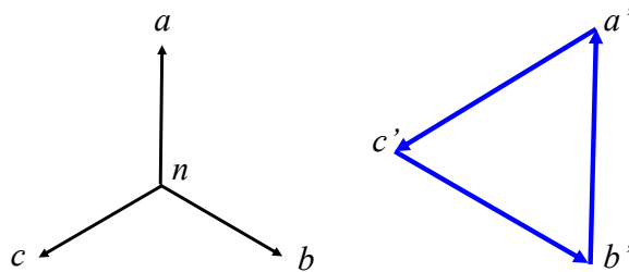
Figure 3.35: Exercise 3.6: Three-phase transformers in Y\Delta configuration.
