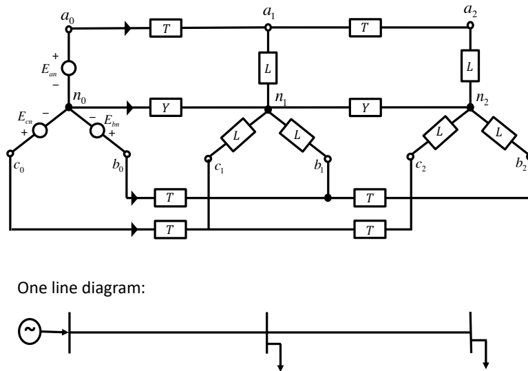
Figure 1.14: Balanced three-phase system in Y configuration (Example 1.4). (Fig change: T \rightarrow t , L \rightarrow l , and Y \rightarrow y .)
