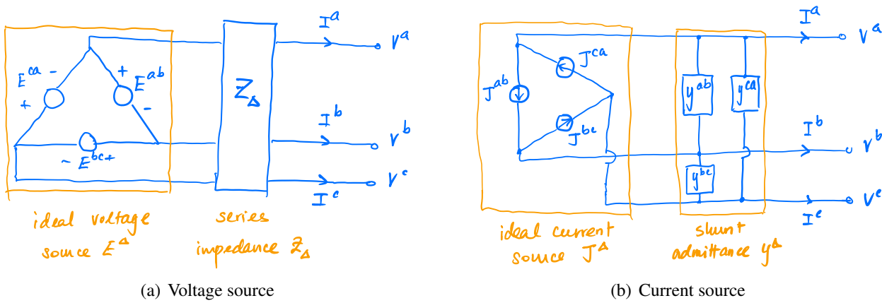
Figure 8.6: Three-wire sources in \Delta configuration. (a) A voltage source. (b) A current source.
