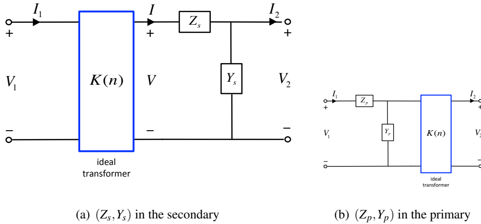
Figure 3.37: Referring (Z_s, Y_s) on the secondary to the primary for an ideal transformer with a complex gain K(n) .
