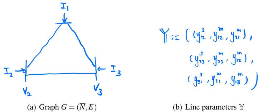
Figure 1.5: One-line diagram for a three-bus network (G, \mathbb{Y}) . It is not a circuit but has an equivalent \Pi circuit model.
