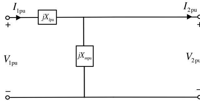
Figure 3.33: Impedance diagram of a three-phase transformer bank.
