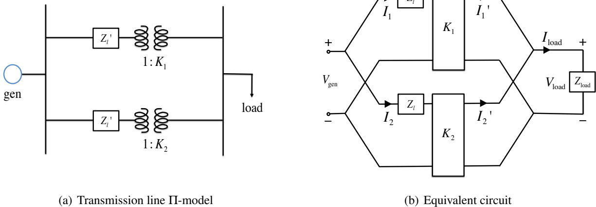
Figure 3.28: Two buses connected in a loop with two parallel transformers.
