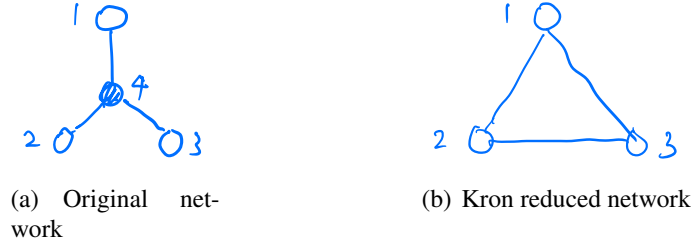
Figure 4.10: Kron reduction: N_{\text{red}} := \{1, 2, 3\} with internal bus 4. While the original network is a tree, the Kron reduced network is fully connected.
